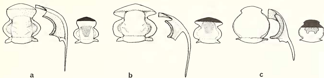
TEXT-FIG. 18. Remopleuridaceans from primitive (a) to advanced (c) types, showing change from inferred natant to impendent hypostomal condition. Smaller sketches show hypostomal position (stippled) in relation to extent of cephalic doublure (black). a, primitive (kainellid) natant type, Elkanaspis (Upper Cambrian; after Ludvigsen 1982, fig. 60). b, conterminant type, Menoparia (Tremadoc; after Ross 1951b, pl. 20). c, impendent type, Remopleurides (mid to late Ordovician). Approximately natural size.
